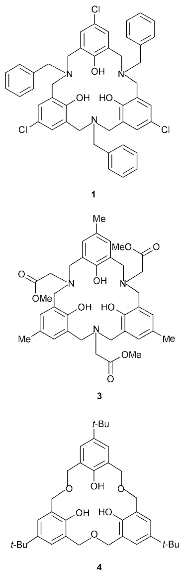
Scheme 1 p -Chloro- N -benzylhexahomotriazacalix[3]arene 1 , p -methyl- N -methoxycarbonylmethylhexahomotriazacalix[3]arene 3 and p - tert -butylhexahomotrioxacalix[3]arene 4 .
